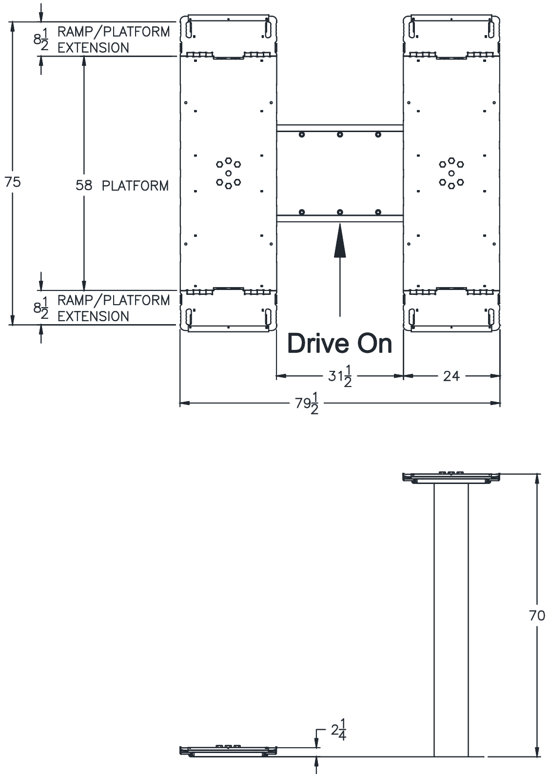
Fig. 1 GENERAL SPECIFICATIONS
