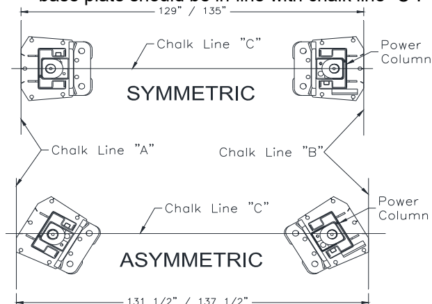
Fig 4 - Layout
