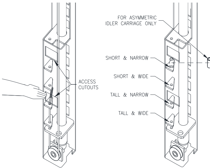
Fig 12a – Cable Attachment Points
