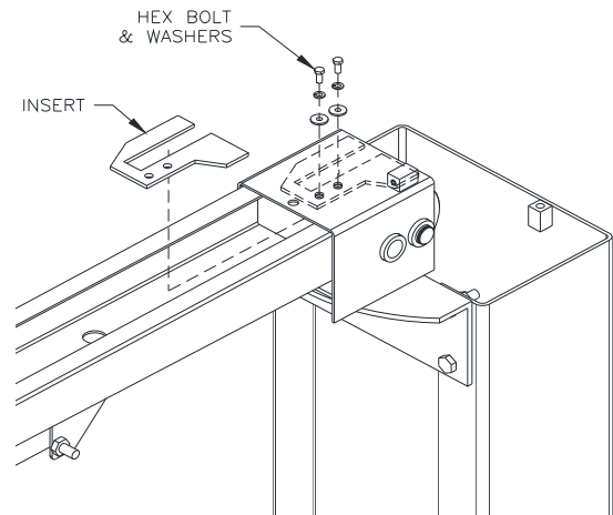
Fig 13 – Cable Trapping
